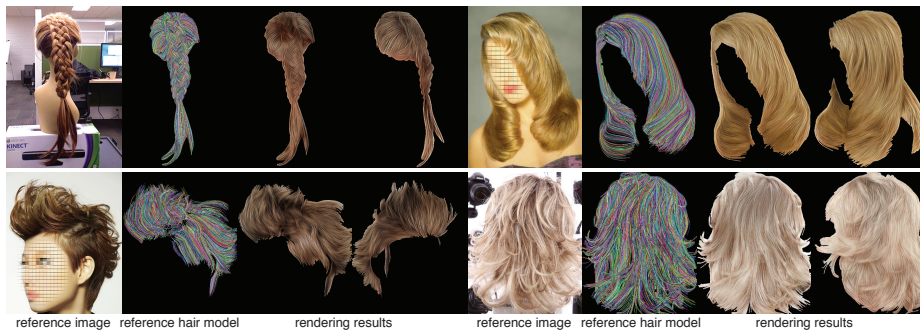
Fig. 1. We propose a real-time hair rendering method. Given a reference image, we can render a 3D hair model with the referenced color and lighting in real-time. Faces in this paper are obfuscated to avoid copyright infringement
