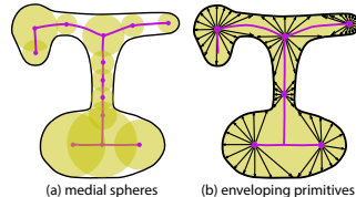
Figure 3: A shape and its medial axis (purple) (a) medial balls (yellow) vs (b) enveloping primitives.
